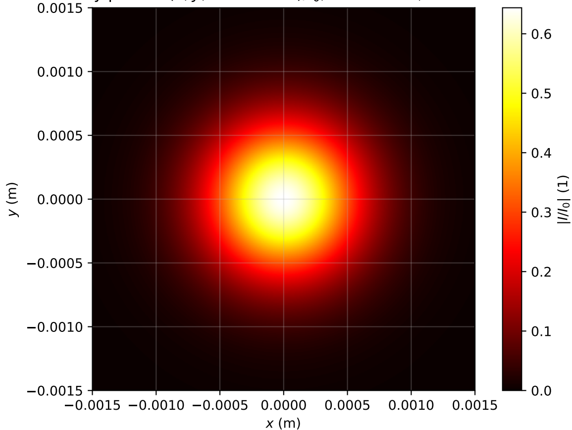
Intensity profile I(x, y, z = 2.309m)/I_0 , Pin=0.4Pcr, artificial time
